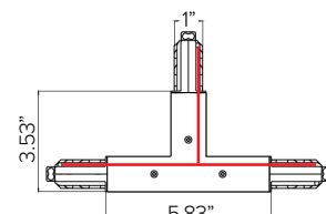
STUCCHI EUROSTANDARD PLUS T – Feed polarity internal right/ground external left.
