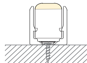
KT09UTC1 (clip) and KT09UTP1 (profile) mounted with mounting screw
