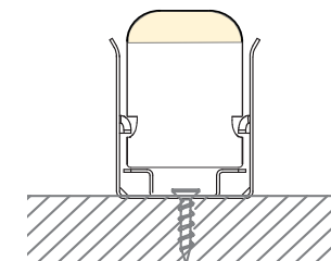
KTUTFP2 (flex profile) mounted with mounting screw
